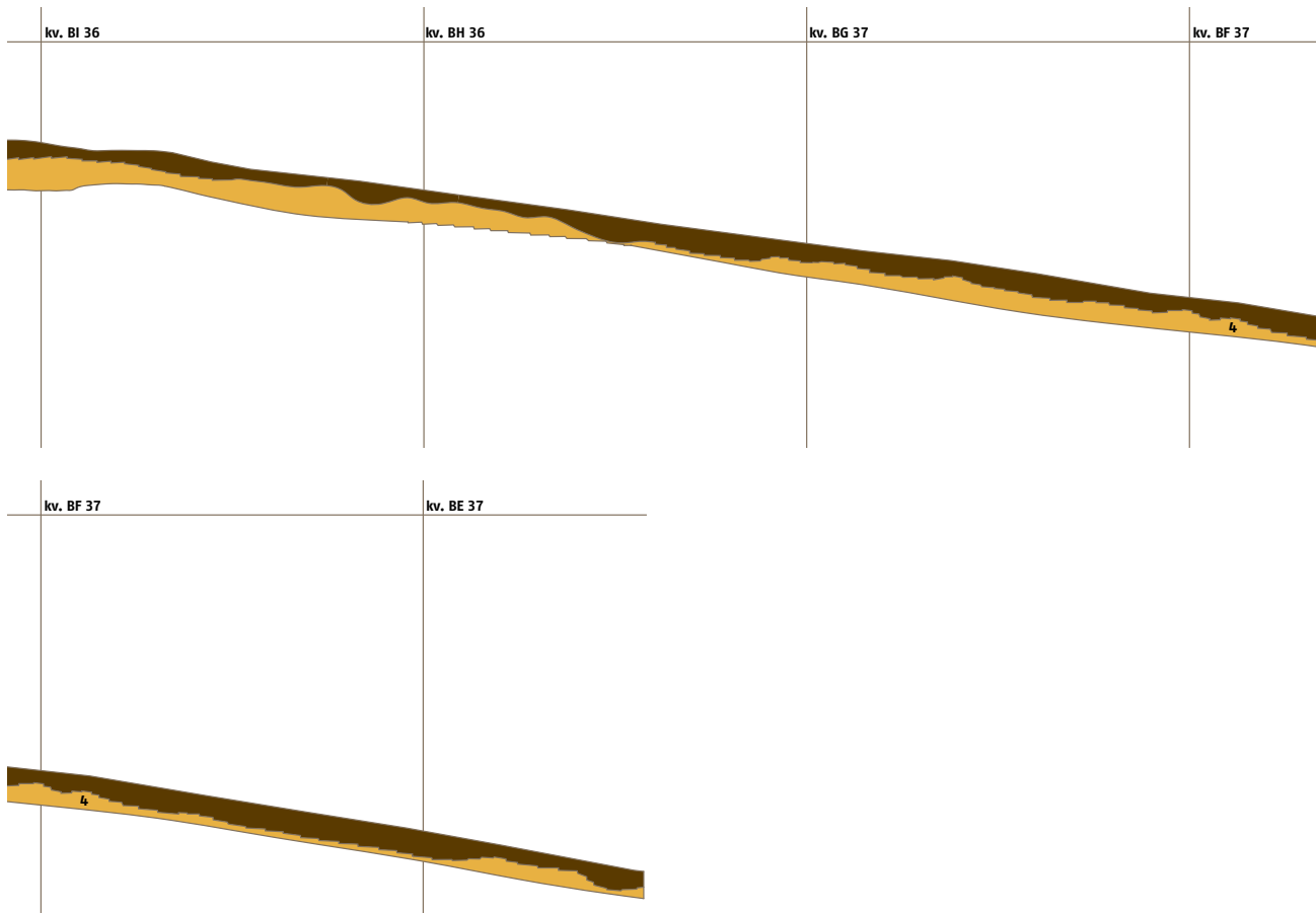
39 Presek 11, M 1:100.
